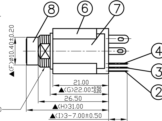
M12XP1.0 METRIC THREAD
