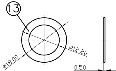
WASHER
