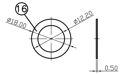
WASHER
