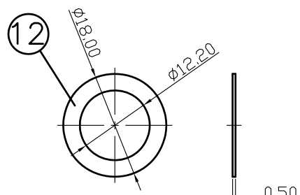
WASHER
