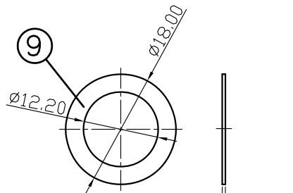
WASHER
