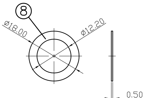
WASHER
