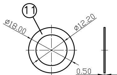
WASHER
