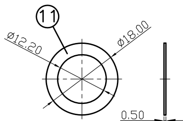
WASHER
