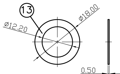
WASHER
