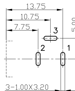
Pin Hole Layout (Jack Bottom View)
