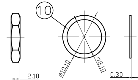
WASHER
