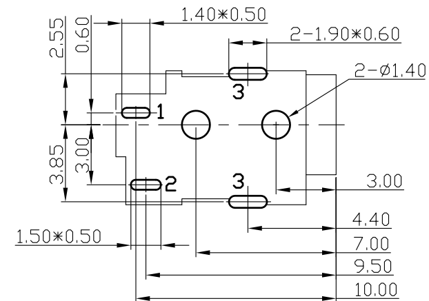
Pin Hole Layout (Jack Bottom View)
