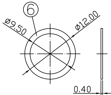
Washer
