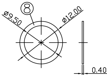
Washer
