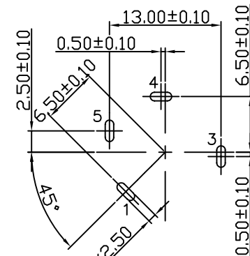
Pin Hole Layout (Jack Bottom View)
