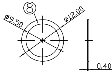
Washer
