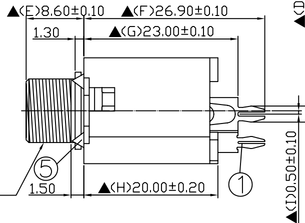
Ø3/8"X32W METRIC THREAD
