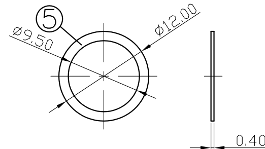
WASHER
