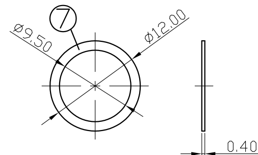
WASHER
