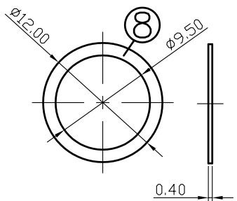
WASHER
