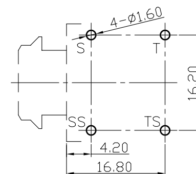
Pin Hloe Layout (Jack Bottom View)
