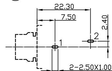
Pin Hole Layout (Jack Bottom View)
