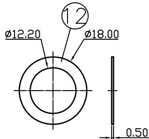
WASHER
