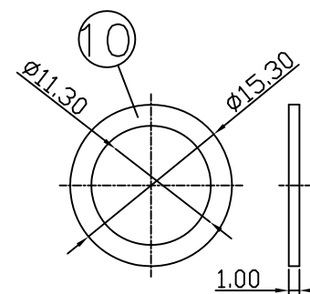
WASHER
