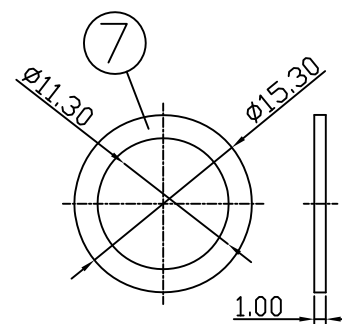
WASHER
