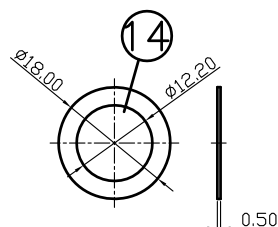
WASHER
