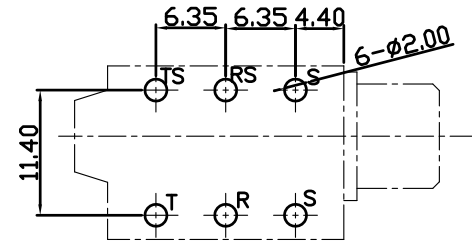
Pin Hole Layout (Jack Bottom View)
