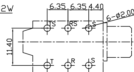
Pin Hole Layout (Jack Bottom View)
