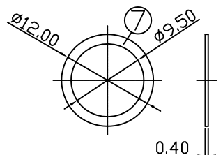
WASHER
