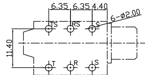
Pin Hole Layout (Jack Bottom View)
