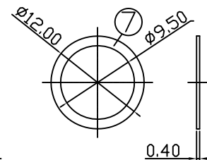
WASHER
