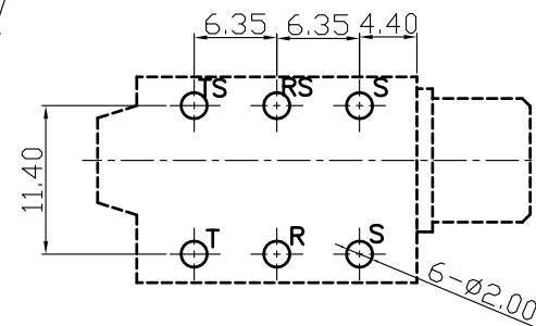
Pin Hole Layout (Jack Bottom View)
