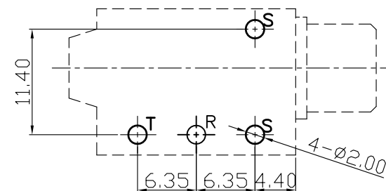
Pin Hole Layout (Jack Bottom View)
