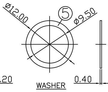
WASHER
