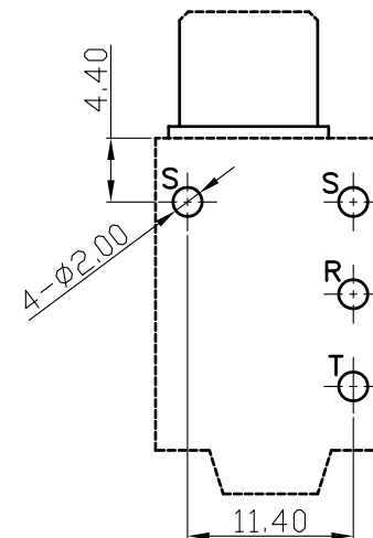
Pin Hole Layout (Jack Bottom View)
