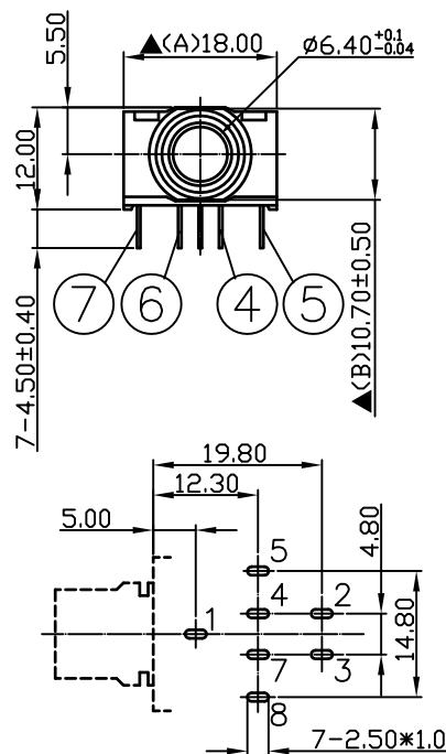
Pin Hole Layout (Jack Bottom View)
