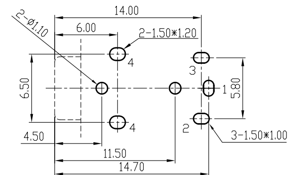
Pin Hole Layout (Jack Bottom View)
