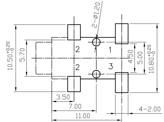
Pin Hole Layout (Jack Bottom View)
