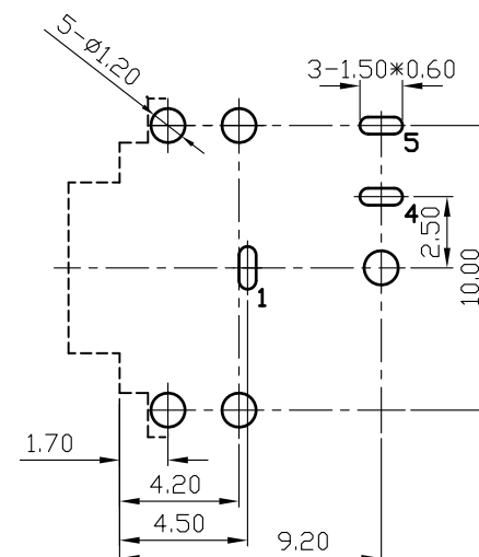
Pin Hole Layout (Jack Bottom View)
