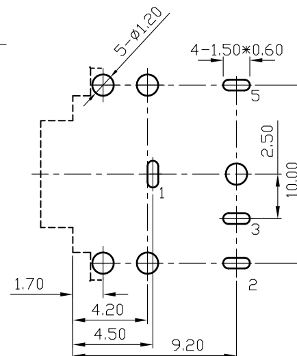
Pin Hole Layout (Jack Bottom View)
