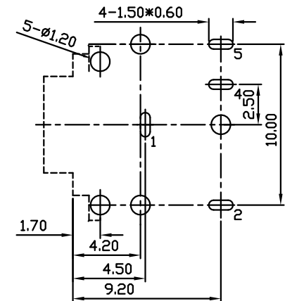
Pin Hole Layout (Jack Bottom View)
