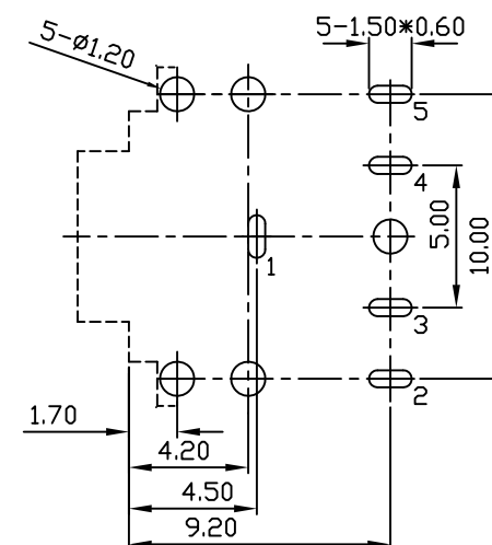
Pin Hole Layout (Jack Bottom View)
