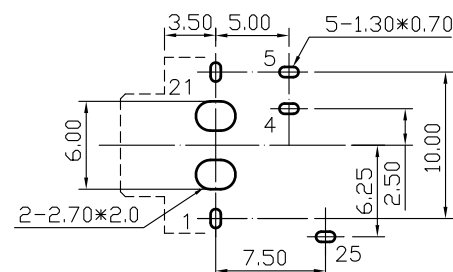
Pin Hole Layout (Jack Bottom View)
