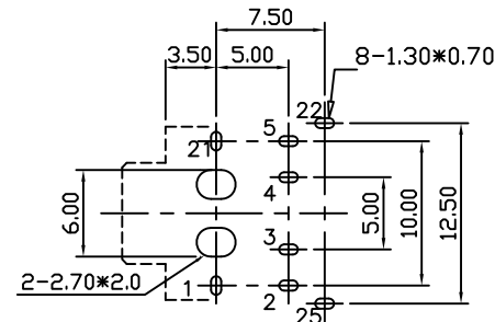
Pin Hole Layout (Jack Bottom View)
