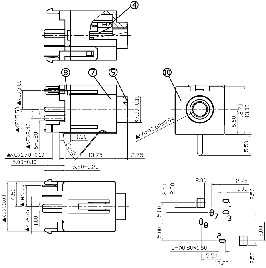
Pin Hole Layout (Jack Bottom View)
