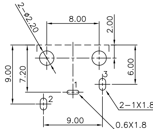
Pin Hole Layout (Jack Bottom View)
