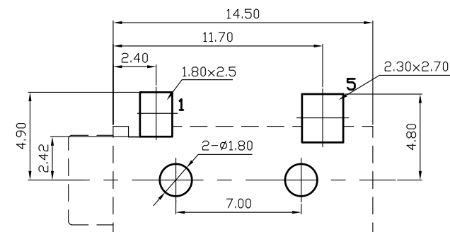
Pin Hole Layout (Jack Bottom View)
