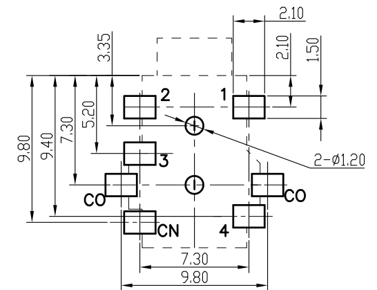
Pin Hole Layout (Jack Bottom View)
