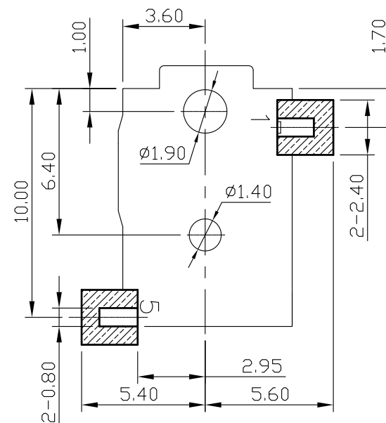
Pin Hole Layout (Jack Bottom View)
