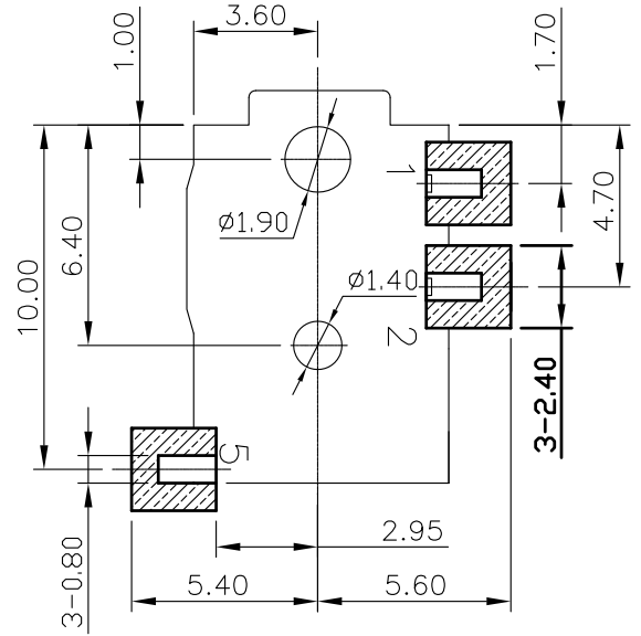
Pin Hole Layout (Jack Bottom View)
