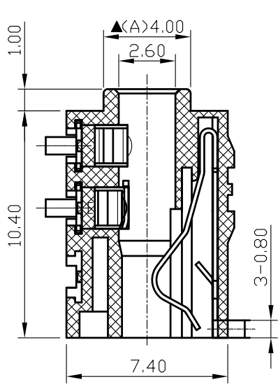
SEC: C-C
