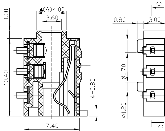
SEC: C-C
