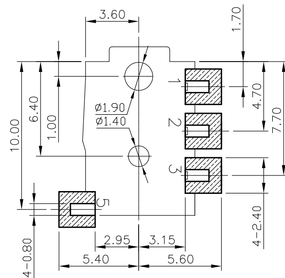
Pin Hole Layout (Jack Bottom View)
