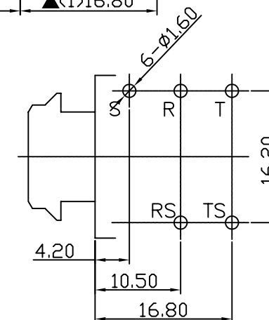
Pin Hole Layout (Jack Bottom View)
