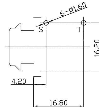
Pin Hole Layout (Jack Bottom View)
