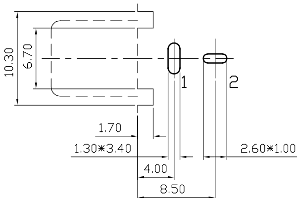
Pin Hole Layout (Jack Bottom View)
